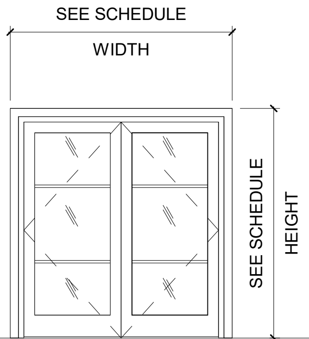
DOOR TYPE E2 - DBL SWING W/ LITE LOCATED AT WEIST ESTATE KITCHEN & DINING HALL) (DOORS 400.1, 418.4, 418.5, & 418.6)
