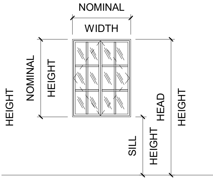
WINDOW TYPE B1 - 2 PANEL CASEMENT LOCATED AT SCREENED PORCH (WINDOWS 602.A, 602.B, 602.C)
