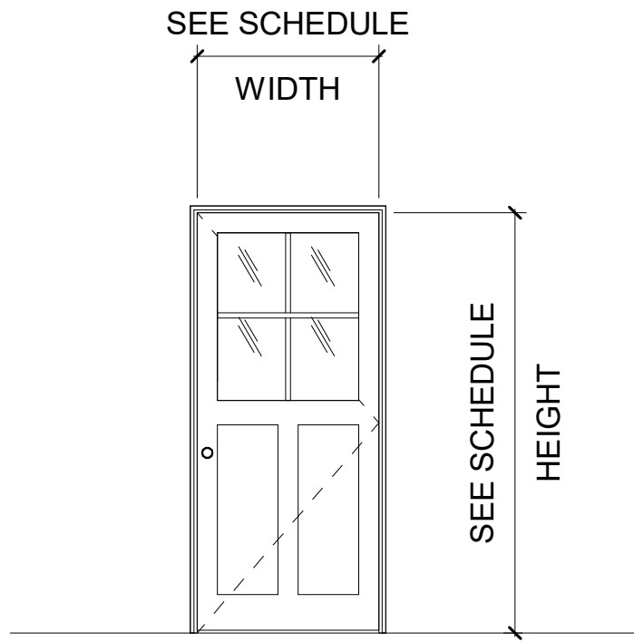
DOOR TYPE A3 - SGL SWING HALF LITE PANEL LOCATED AT POOL HOUSE UNITS & LAUNDRY ROOM (DOORS 304.1, 307.2, 312.2, 316.2)
