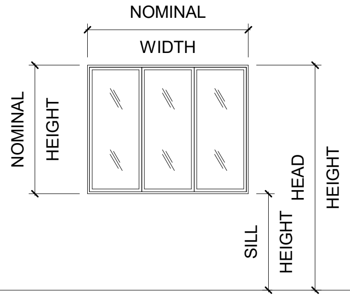
WINDOW TYPE C1 - FIXED MULTI-PANEL LOCATED AT WEIST ESTATE OUTDOOR HALLWAY (WINDOWS 400.C & 400.F)
