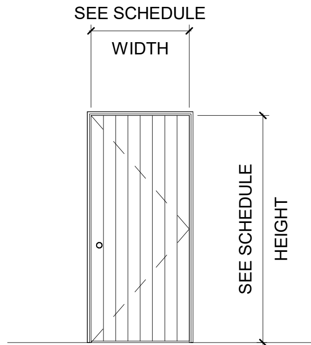
DOOR TYPE A5 - SGL SWING PLANK PANEL LOCATED AT POOL ROOM & POOL HOUSE (DOORS 300.1, 301.1, 302.1)
