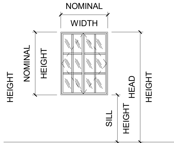
WINDOW TYPE B1 - 2 PANEL CASEMENT LOCATED AT POOL HOUSE UNITS (WINDOWS 313.A, 317.A)
