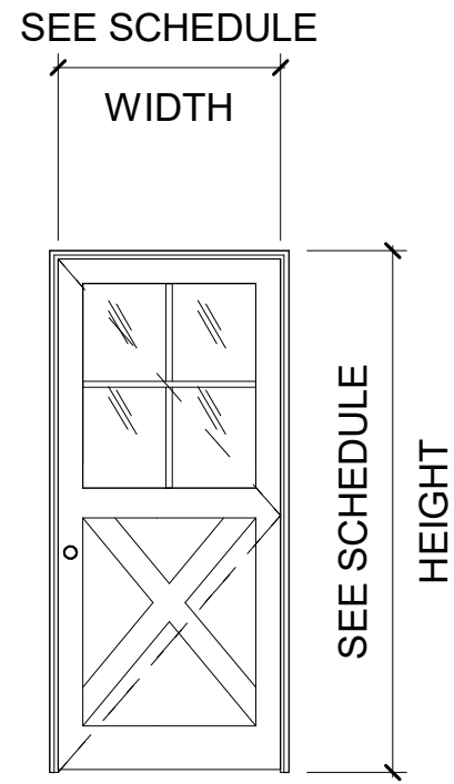
DOOR TYPE A3 - SGL SWING HALF LITE PANEL (DOOR 706.1)
