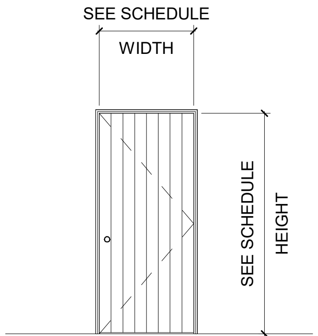
DOOR TYPE A5 - SGL SWING PLANK PANEL LOCATED AT CHAPEL ENTRY DOOR (DOOR 501.1)
