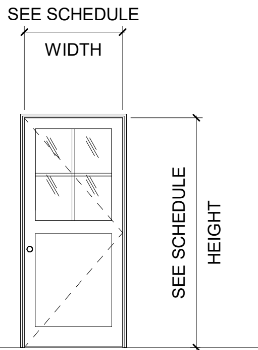
DOOR TYPE A3 - SGL SWING HALF LITE PANEL LOCATED AT WEIST ESTATE UNITS & LAUNDRY ROOM (DOORS 407.1, 410.2, 413.2, 416.2)
