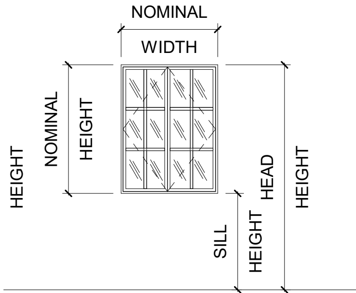
WINDOW TYPE B1 - 2 PANEL CASEMENT (WINDOW 701.A)
