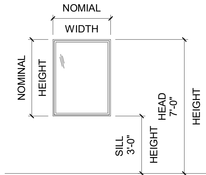
WINDOW TYPE A1 - FIXED LOCATED AT CHAPEL ENTRY (WINDOW 500.A)
