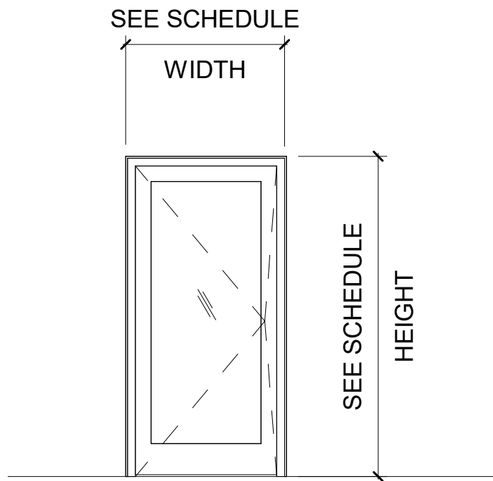
DOOR TYPE B2 - PIVOT DOOR WITH LITE LOCATED AT CHAPEL ENTRY DOOR (DOOR 500.1)
